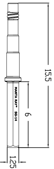
SG-14 SHANK
